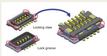
Mating of MLC Series 5-pin connector (page 27)
