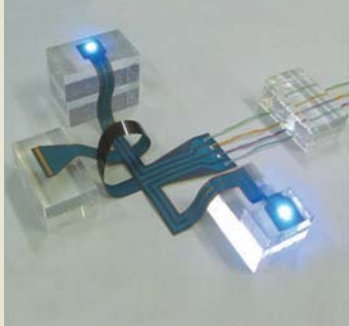
Example of LED surface mounting onto Ag printing pattern by soldering. (page 42)
