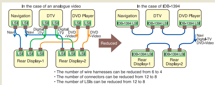
Reductions in wire harnesses thanks to IDB-1394 (page 18)
